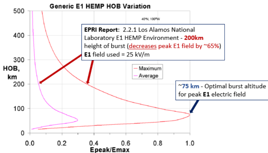
Figure 2-6. Sample E1 HEMP HOB variation. This shows the HOB variation, for a typical device, for the highest E1 peak seen over the full exposed region (red line), and for the average E1 Peak – averaged over all the exposed area. The E1 peak levels are plotted as a fraction of the absolute maximum E1 HEMP for all burst heights (it occurs about HOB=75 km in this case).
